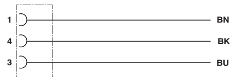
Contact assignment of M8 plugs/sockets
