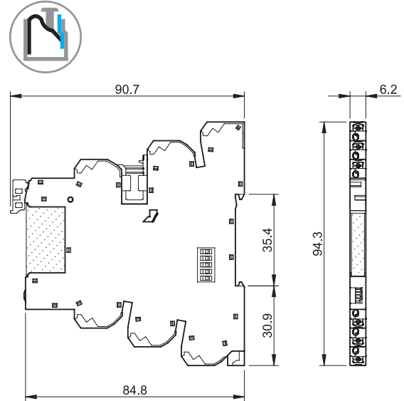
39.90 39.91 Push-in terminal
