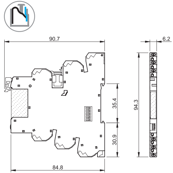
39.90 39.91 Push-in terminal
