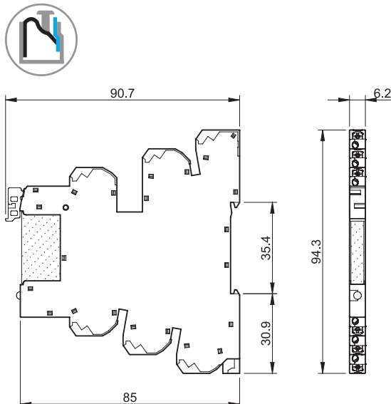
39.70 39.71 Push-in terminal
