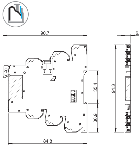
39.90 39.91 Push-in terminal
