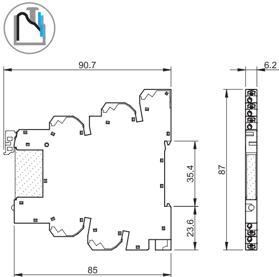
39.00/39.01 39.50/39.51 Push-in terminal
