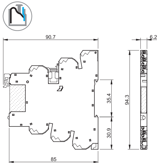
39.90 39.91 Push-in terminal
