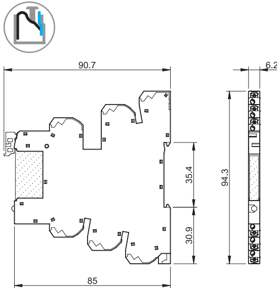
39.70 39.71 Push-in terminal
