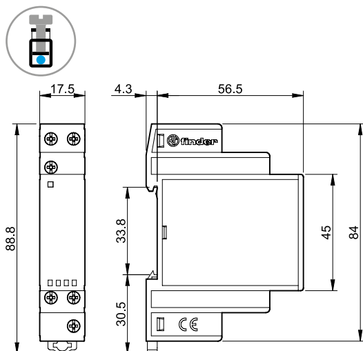
70.61 Screw terminal
