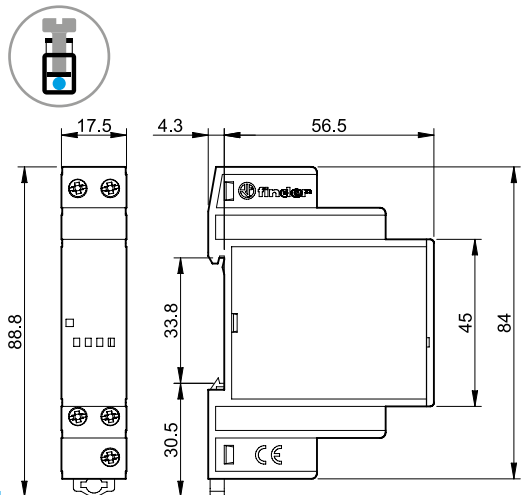
70.11 Screw terminal
