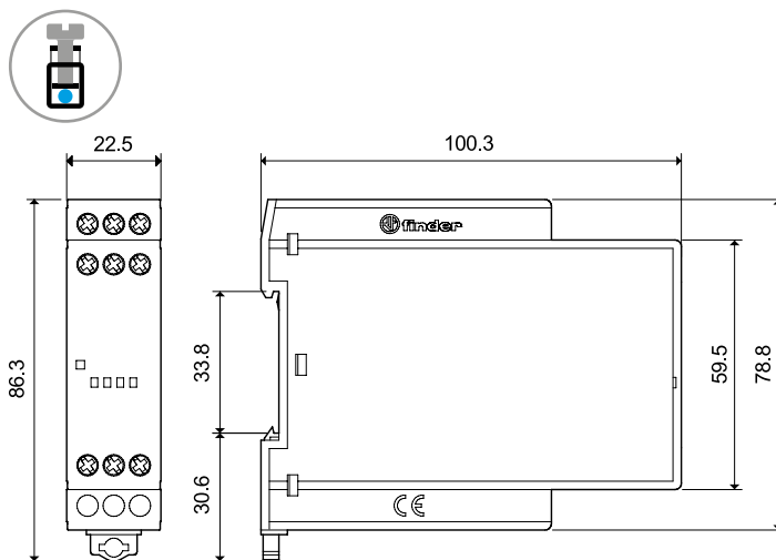
70.62 Screw terminal
