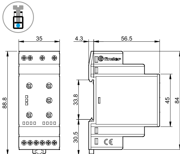
70.42 Screw terminal
