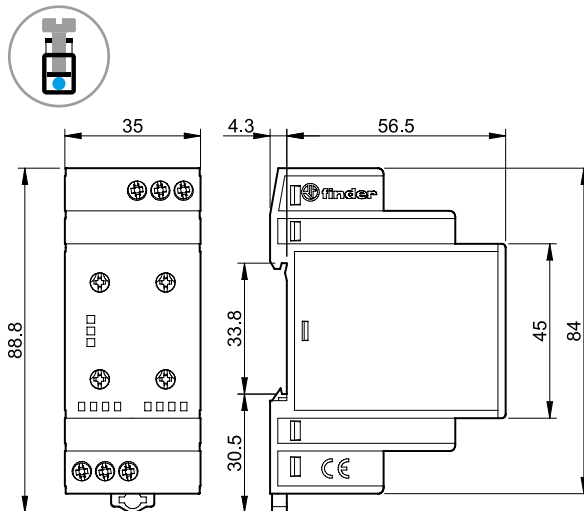
70.42 Screw terminal
